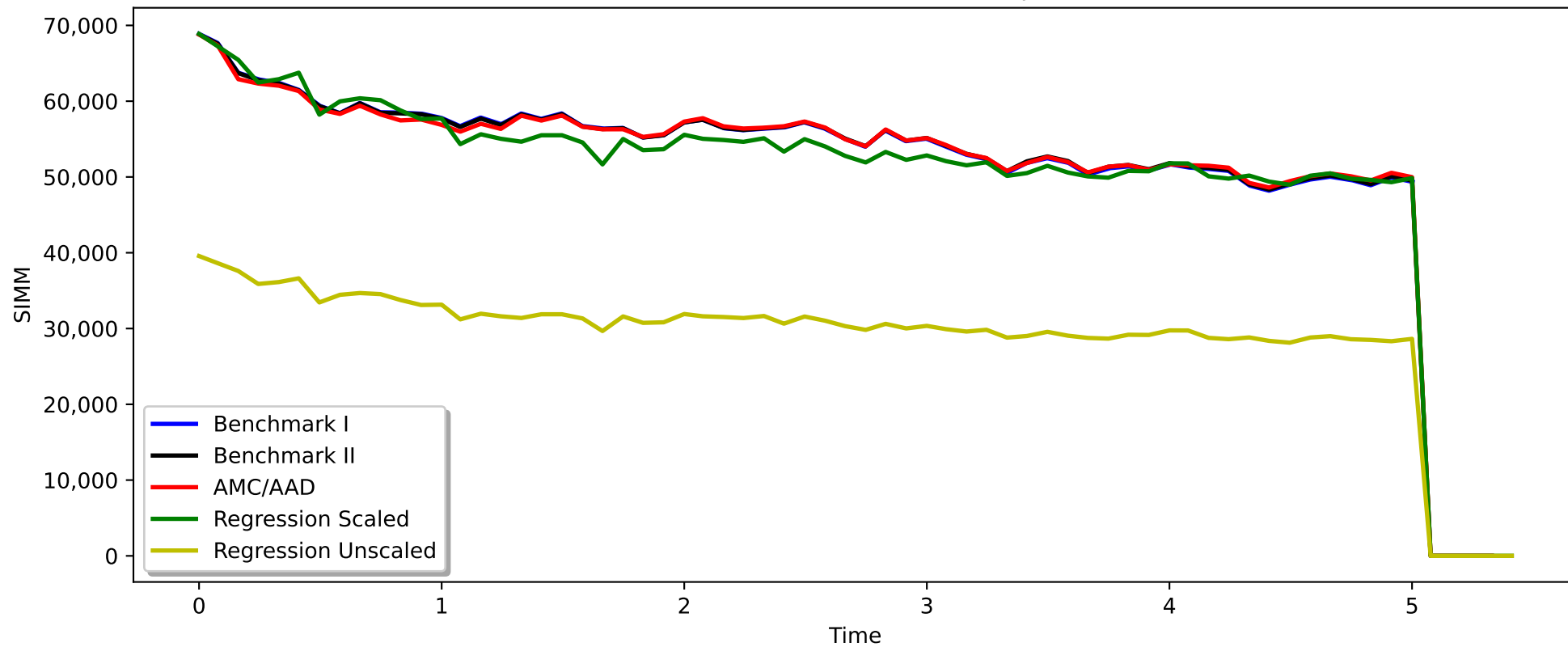
SIMM Evolution Pathwise, Sample 3
