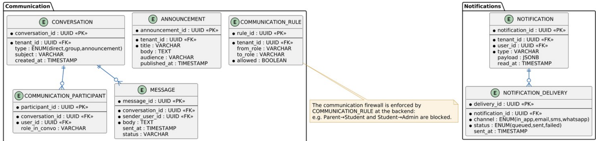
Figure 8 — Communication & Notifications ERD.
