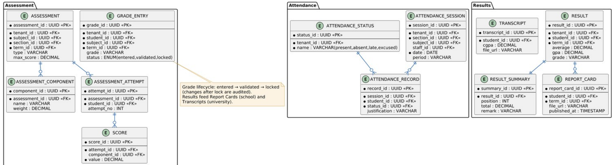
Figure 5 — Academic operations ERD.
