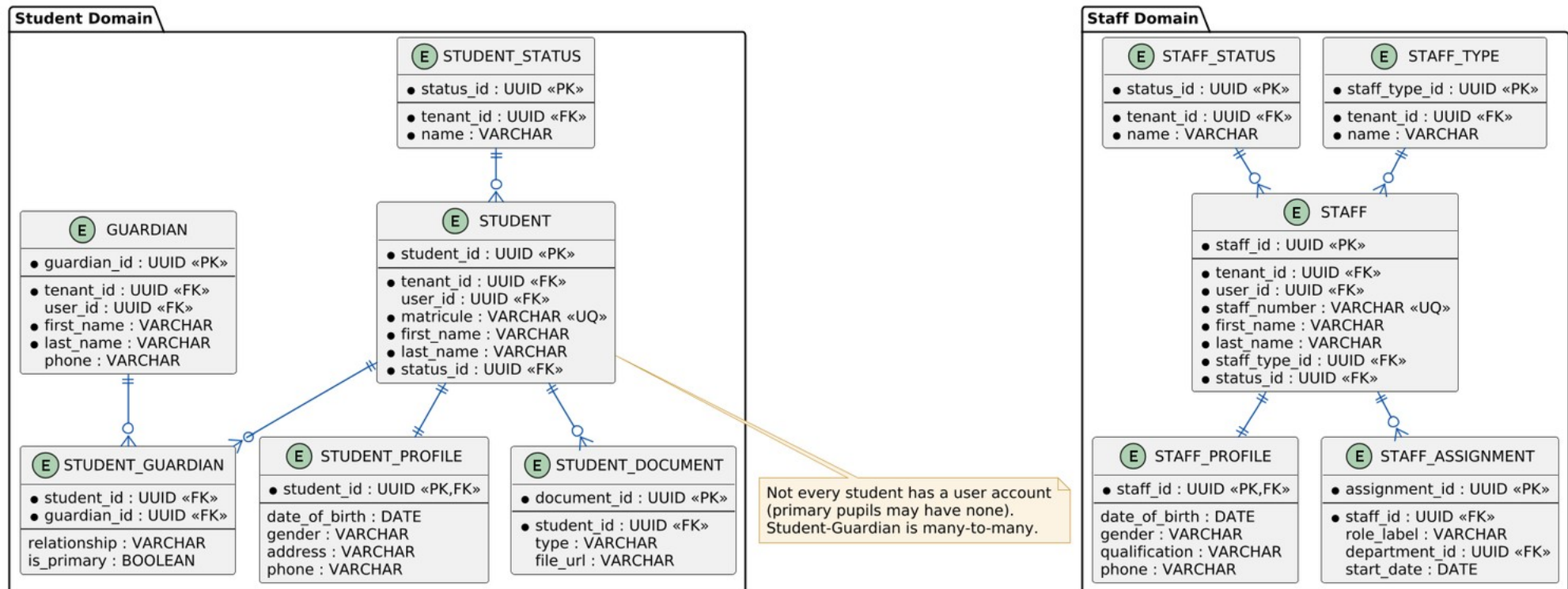
Figure 3 — Student & Staff domains ERD.
