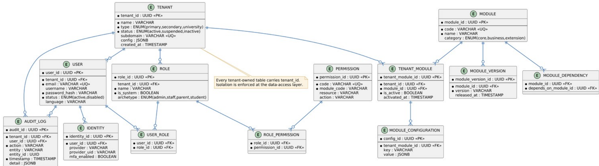
Figure 2 — Core Platform domain ERD.
