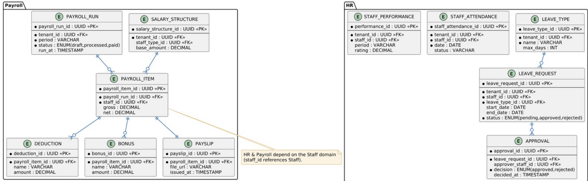
Figure 7 — HR & Payroll domains ERD.
