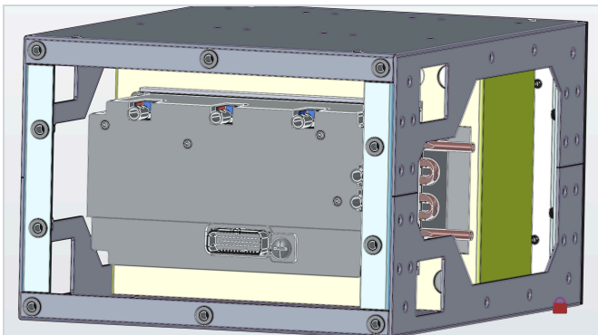
Size 2 DC/DC module: Released design rendering. The 15 kW converter reuses the Size 2 PCBs and power stage; orderable BOMs are available.
