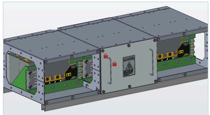
Size 3 high-power enclosure: Design rendering. The up-to-1,200 V, 1,400 A concept uses modular liquid-cooled bays; arc-flash containment analysis is in progress.
