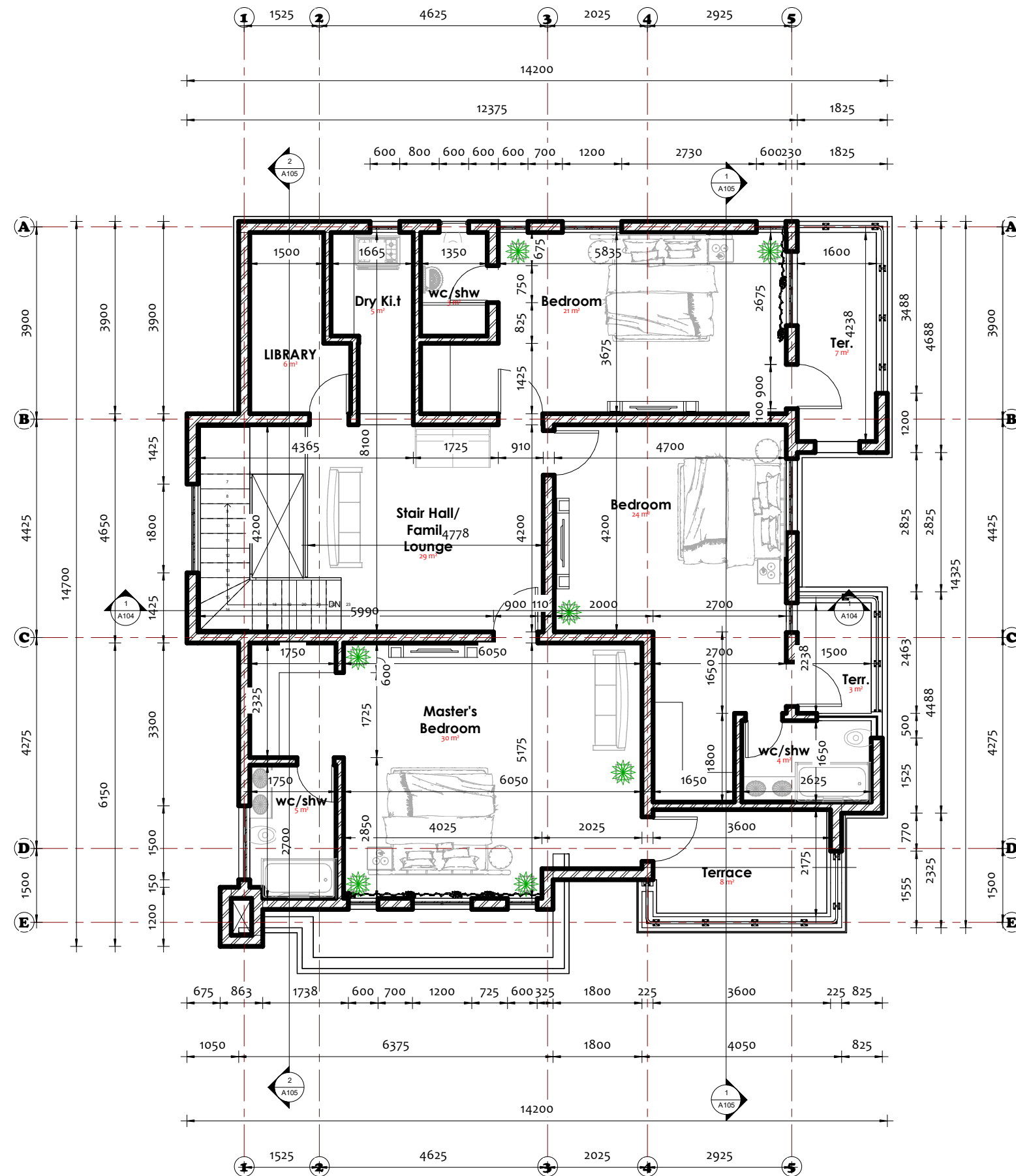
1 02 First Floor 1 : 50
