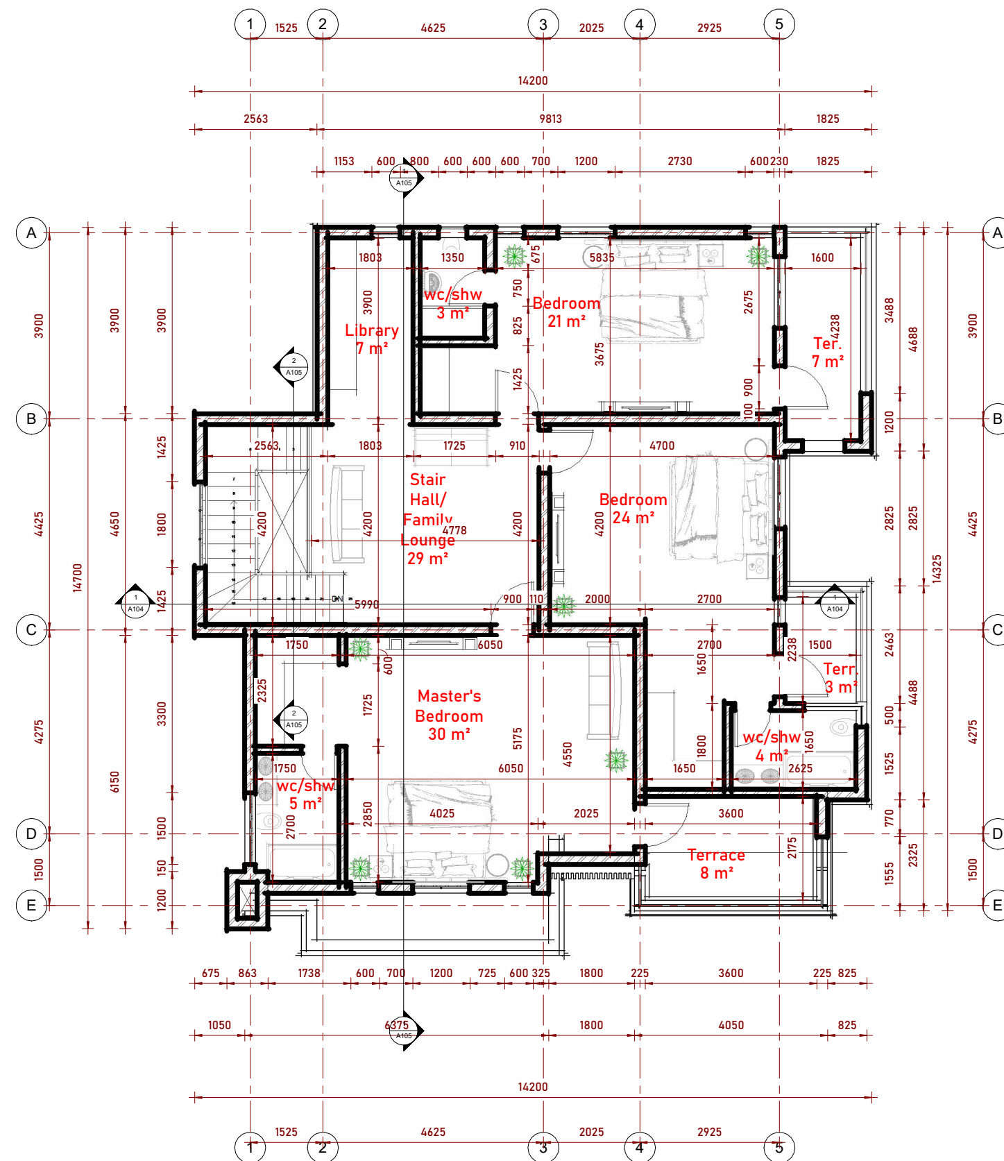
1 02 First Floor 1 : 50
