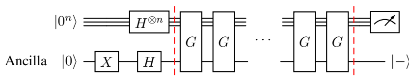
Figure 8: Quantum circuit implementing Grover's algorithm.
