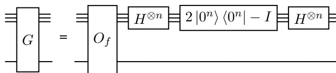
Figure 9: The Grover Operator.
