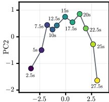
AF-Next L16
