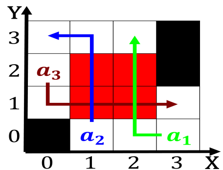
Figure 3: Diversiication in whether new Exhibit sexually other losses
