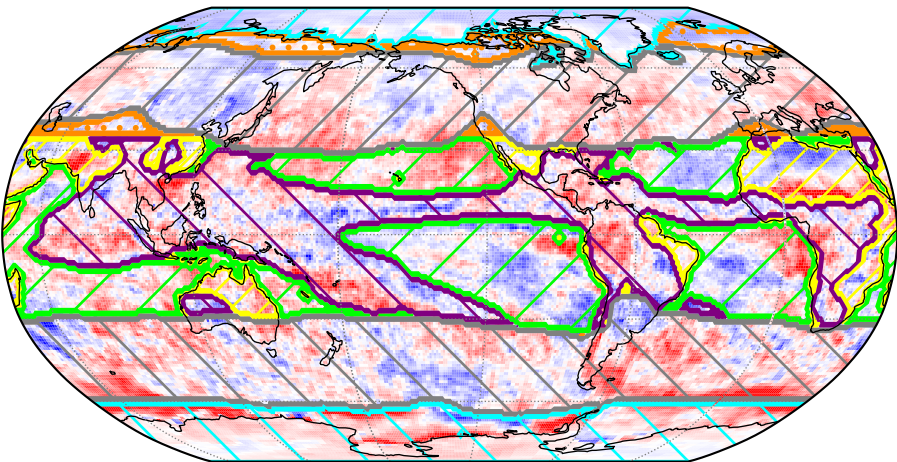
c) SON = 0.41
