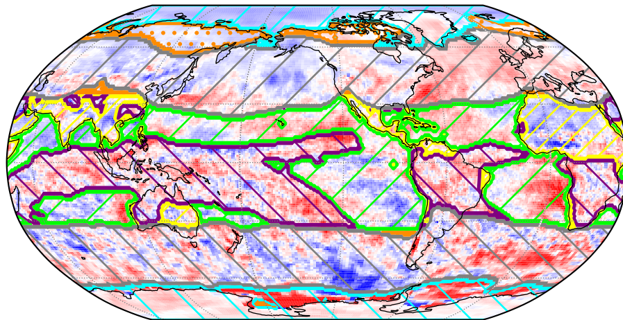
d) DJF = 0.35
