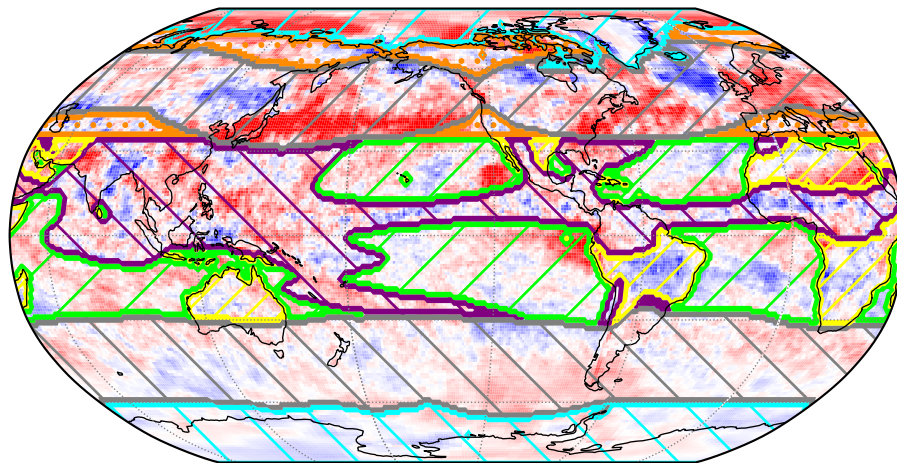
b) JJA = 0.61
