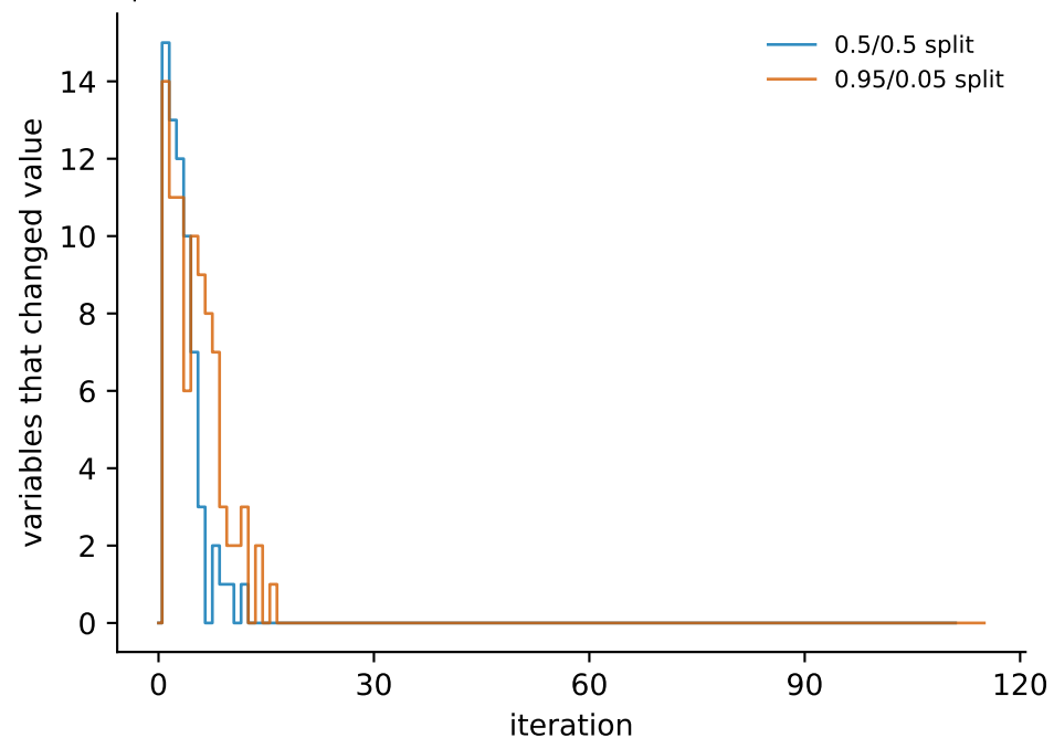
How many variables still change each iteration, under each split
