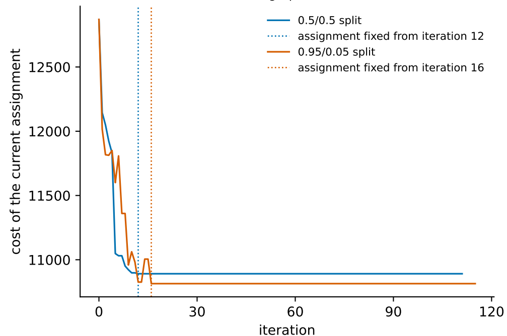
Cost over the run on the same graph (20 nodes, seed 0)
