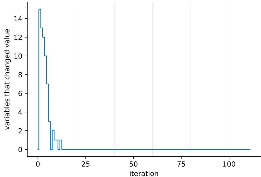
How many of the 20 variables still change each iteration
