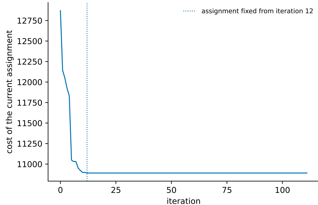
Cost over the run (20 nodes, seed 0, split 0.5/0.5)
