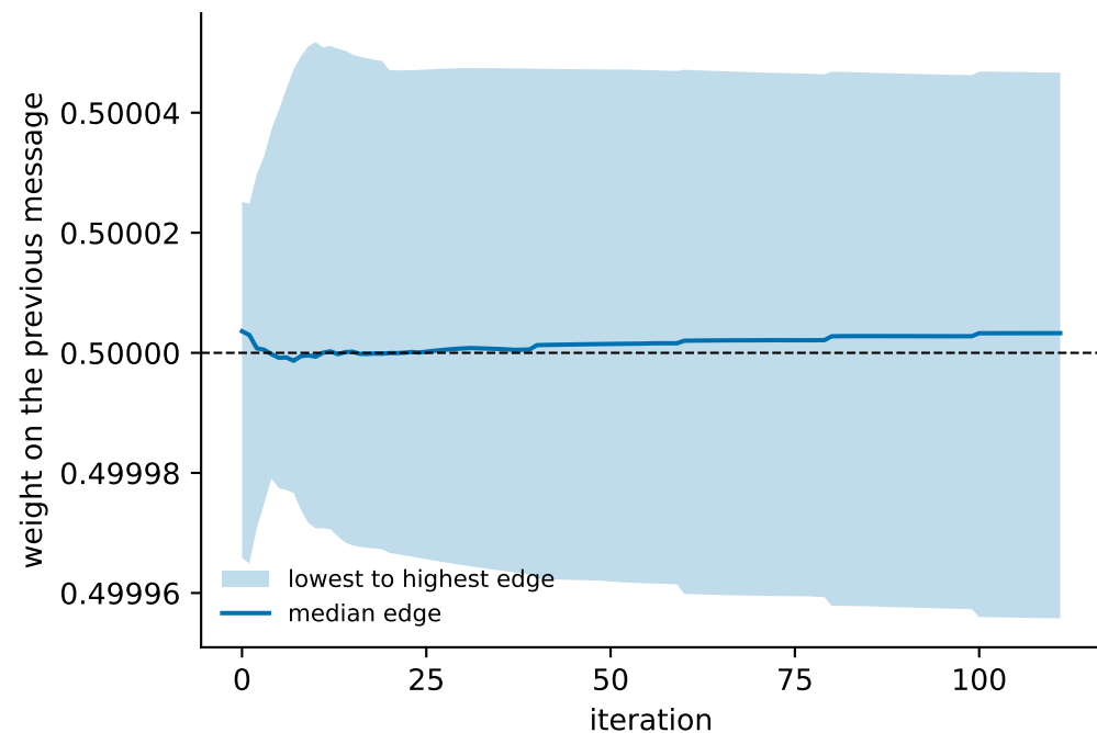
Lowest, median and highest edge at each iteration (20 nodes, seed 0)
