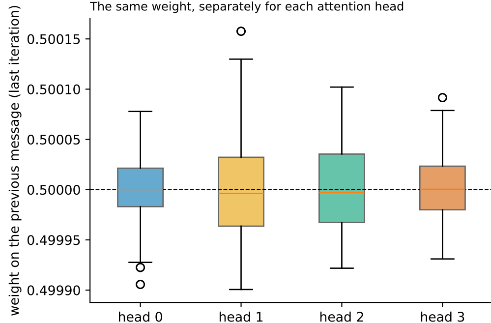
The same weight, separately for each attention head
