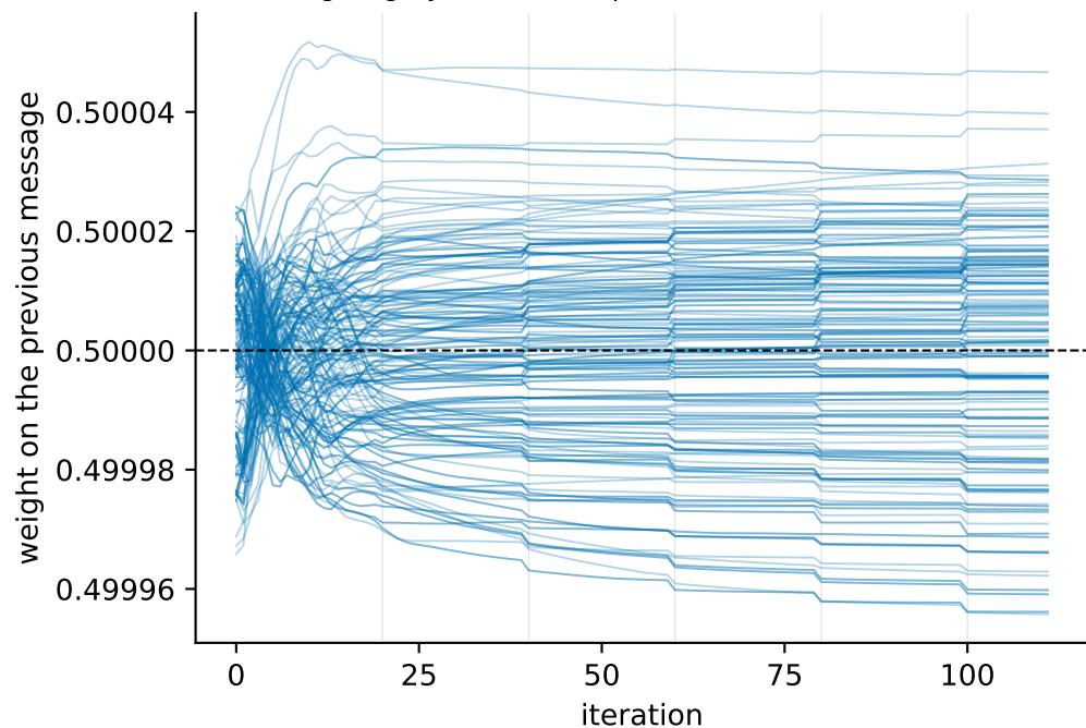
Each edge's damping weight over the run (20 nodes, seed 0, 200 of 352 edges; gray = network update)
