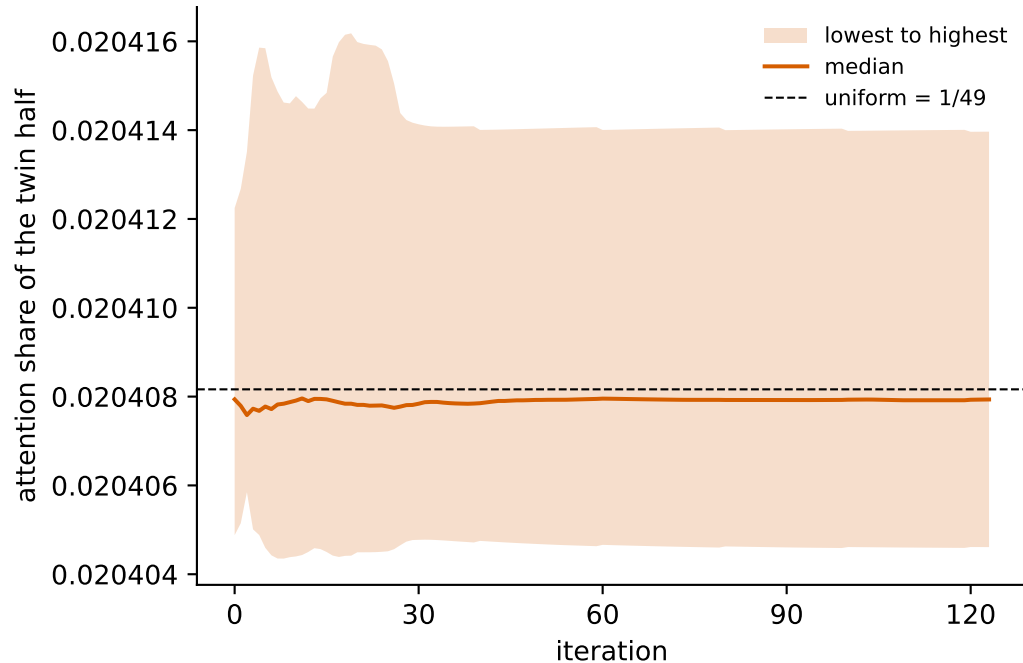
Share given to the twin half over the run, edges with 49 incoming neighbors (2460 twin rows in total, 50 nodes, seed 0)
