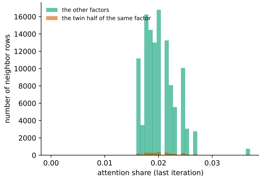
Share given to the twin half over the run, edges with 49 incoming neighbors (2460 twin rows in total, 50 nodes, seed 0)
