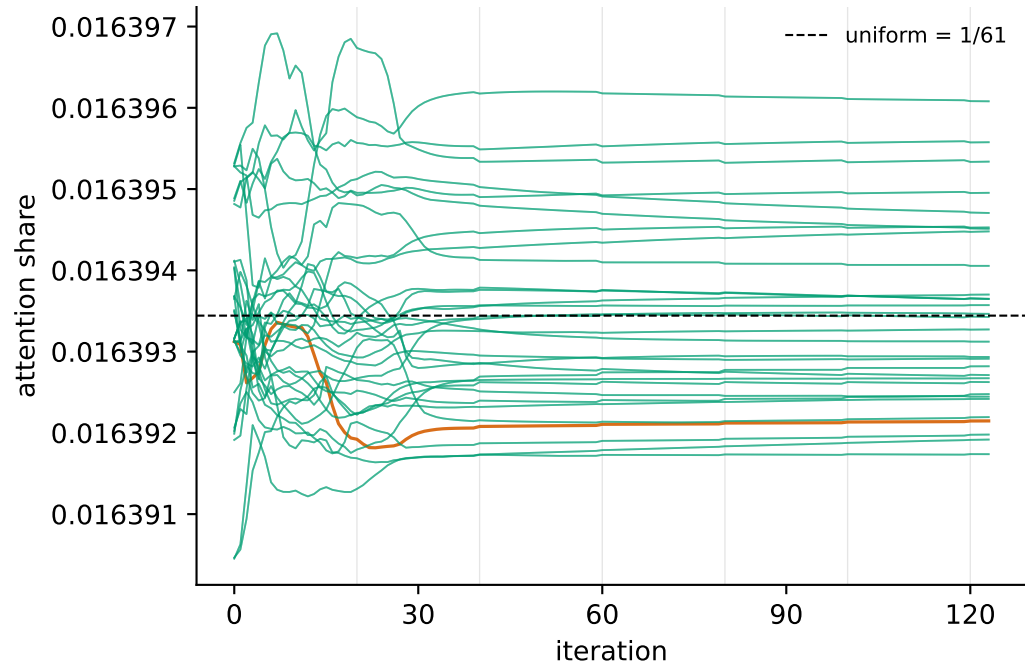
All 61 incoming shares of one edge (50 nodes, seed 0, x17 to f117; red = twin half)
