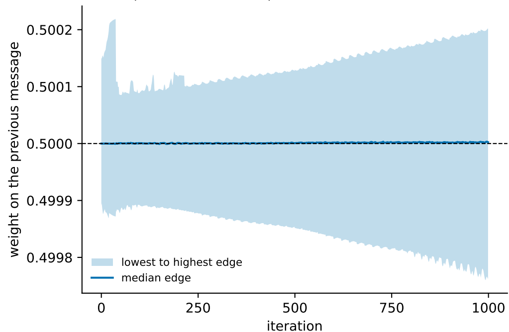
Lowest, median and highest edge at each iteration (50 seeds; a seed drops out once its run stops)
