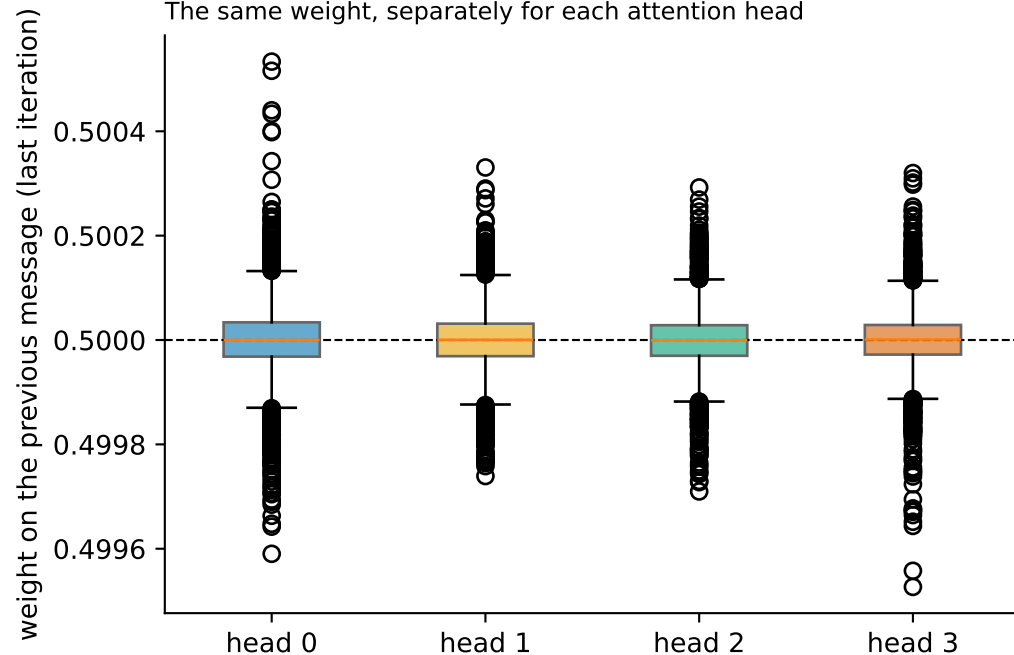
The same weight, separately for each attention head
