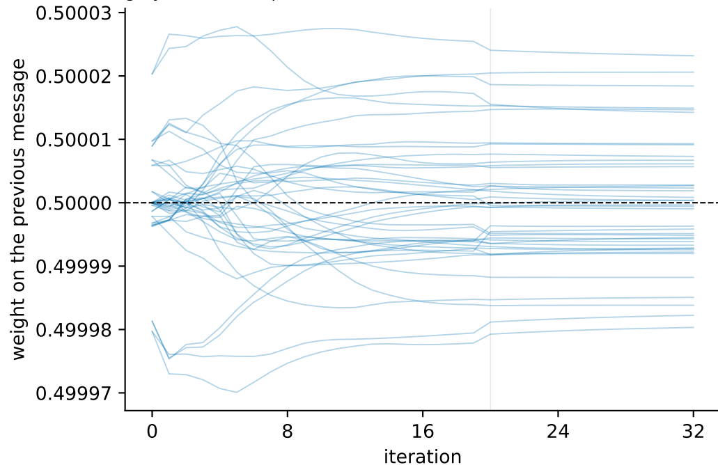
Each edge's damping weight over the run (seed 0, all 40 edges; gray = network update)
