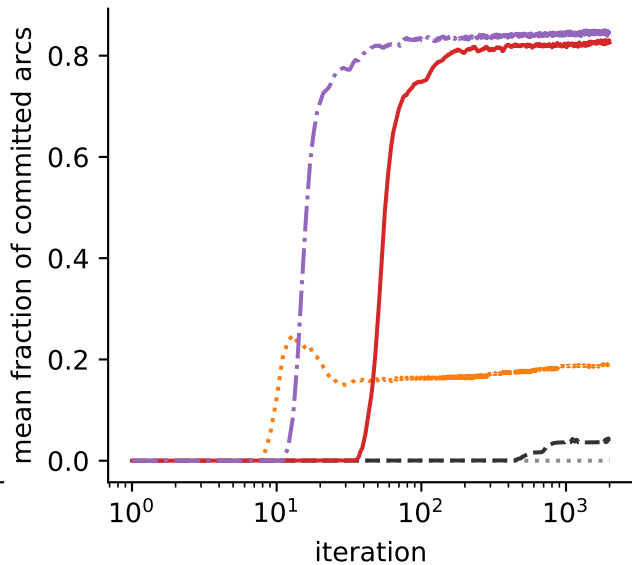
graph coloring, 50 seeds
