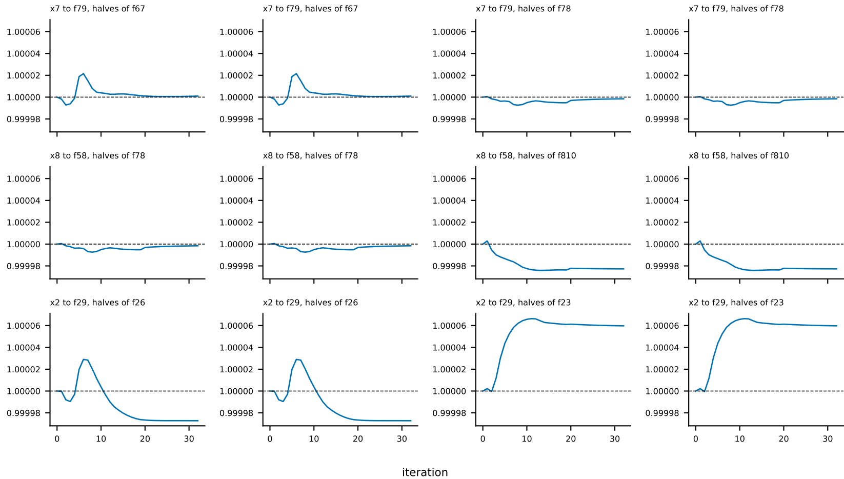
Edge-weight ratio share(half A) / share(half B) over the run, messages sent to variables of degree 2, all 12 pairs (seed 0, same y range in every degree file, panels ordered from least to most asymmetric at the end)
