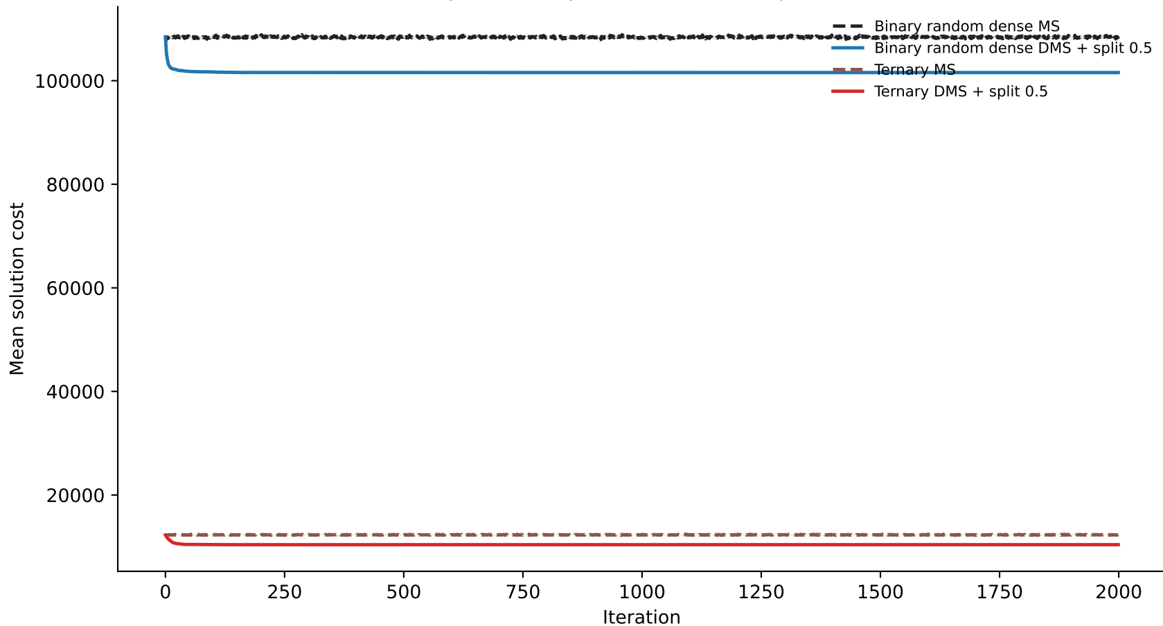
Dense binary vs ternary, MS and DMS + split 0.5, 50 seeds
