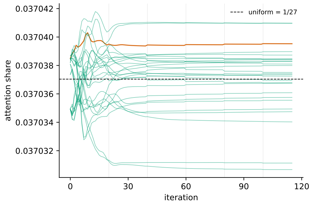
All 27 incoming shares of one edge (20 nodes, seed 0, x19 to f219; red = twin half)
