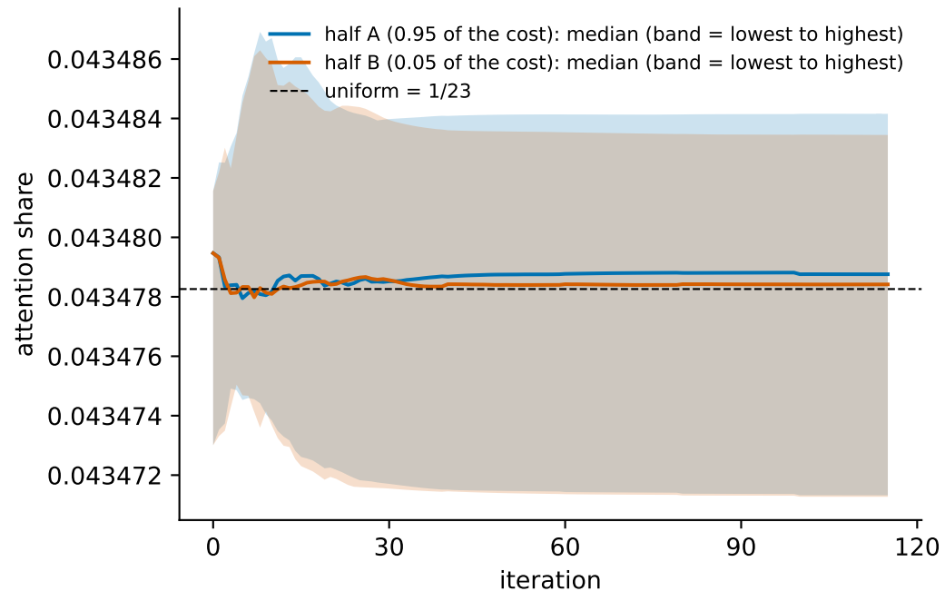
Share of half A against half B over the run, messages with 23 incoming neighbors (792 of 3036 pairs, 20 nodes, seed 0)
