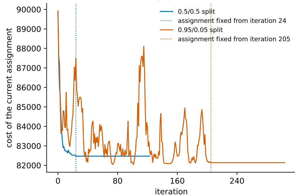
Cost over the run on the same graph (50 nodes, seed 0)
