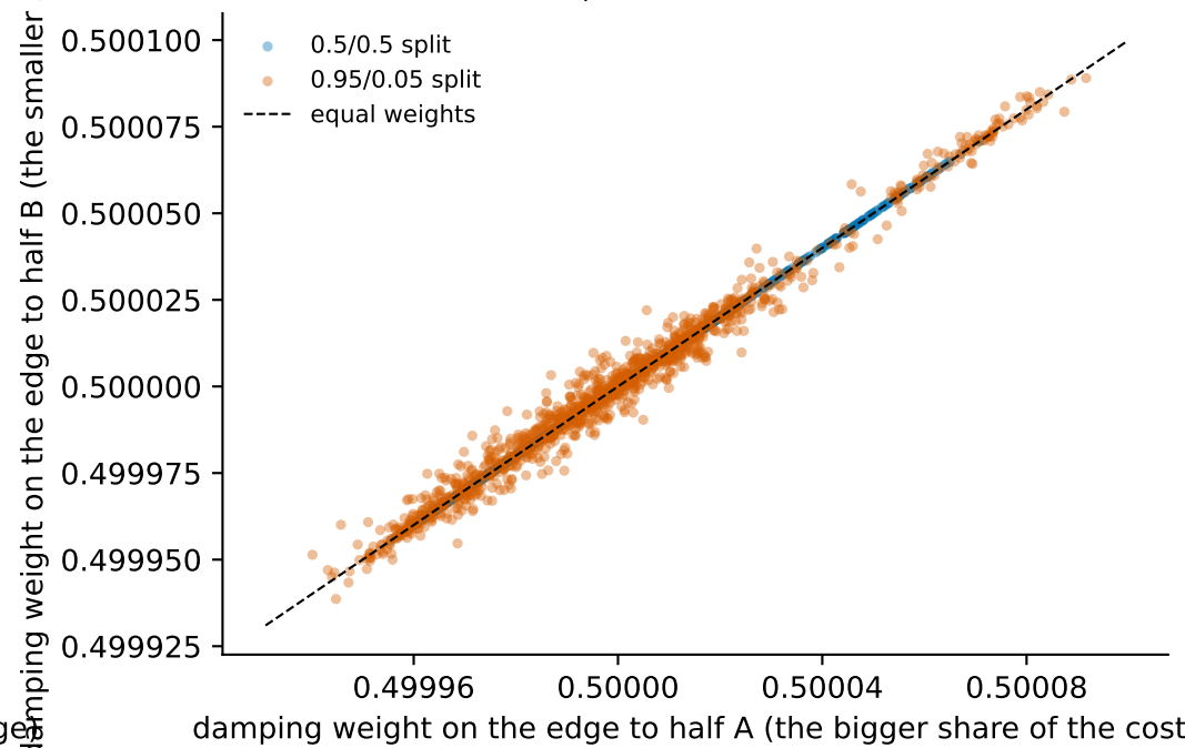
Damping weight of the two edges of each split factor at the last iteration, under each split
