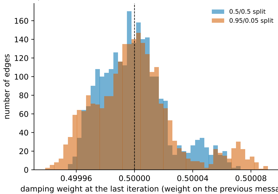
Damping weight of every edge at the last iteration, under each split
