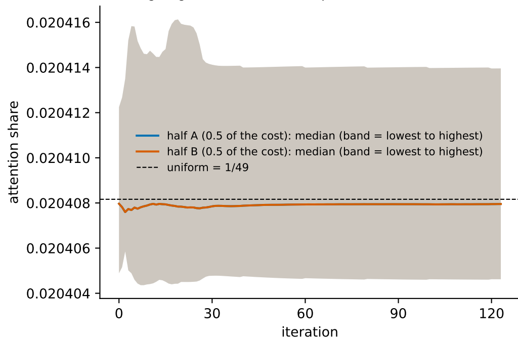
Share of half A against half B over the run, messages with 49 incoming neighbors (8400 of 59312 pairs, 50 nodes, seed 0)
