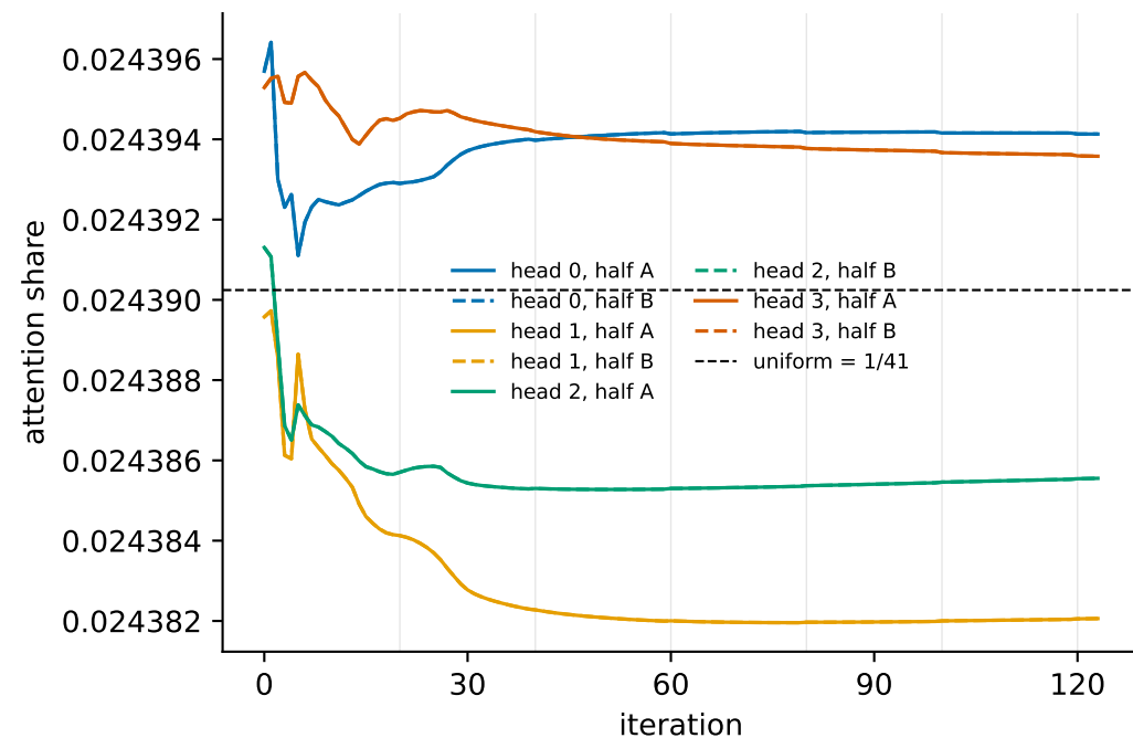
The pair whose shares drifted apart the most (50 nodes, seed 0, x1 to f14, halves of f15; solid = half A, dashed = half B)
