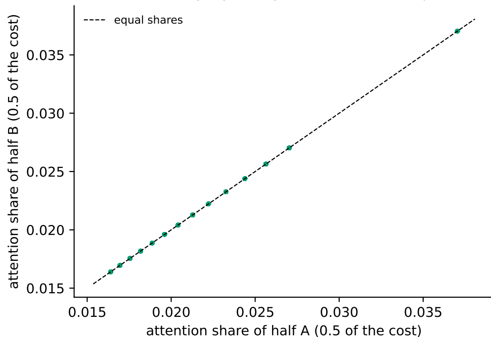
Edge weights: attention share of the two halves of a factor inside the same outgoing message, last iteration (59312 pairs)
