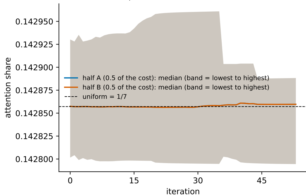
Share of half A against half B over the run, messages with 7 incoming neighbors (2208 of 7280 pairs, 50 seeds; a seed drops out once its run stops)
