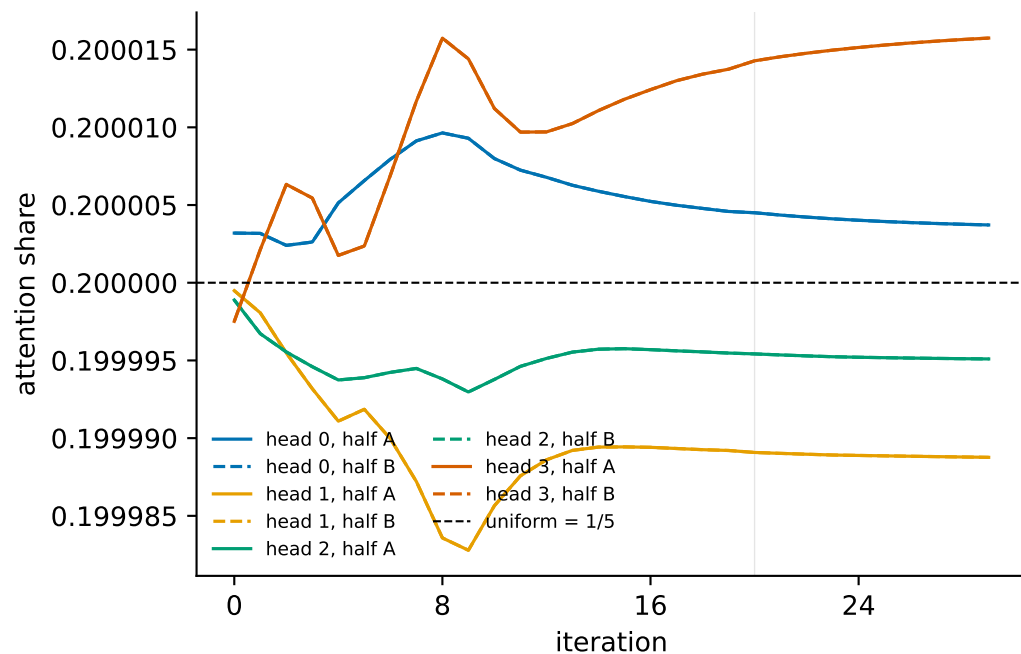
The pair whose shares drifted apart the most (seed 0, x2 to f26, halves of f29; solid = half A, dashed = half B)
