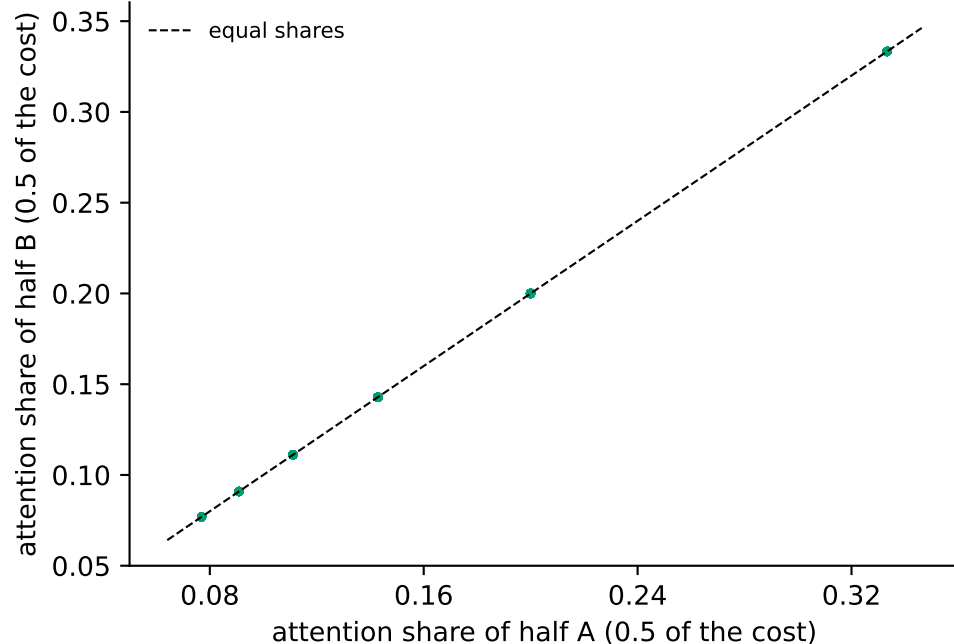
Edge weights: attention share of the two halves of a factor inside the same outgoing message, last iteration (7280 pairs)
