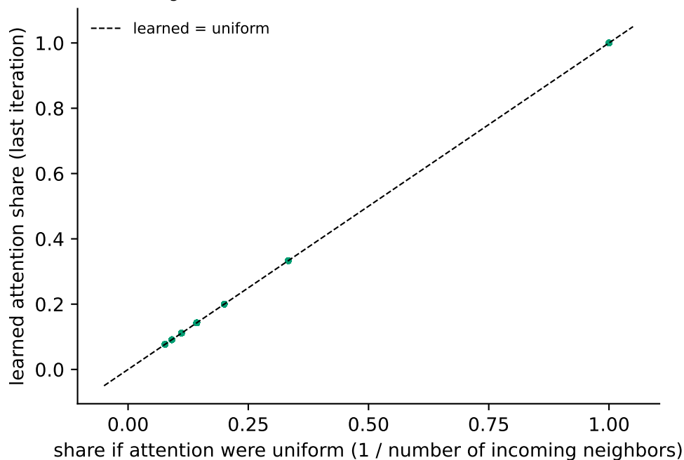
Attention share of each incoming neighbor against uniform (17448 neighbor rows)
