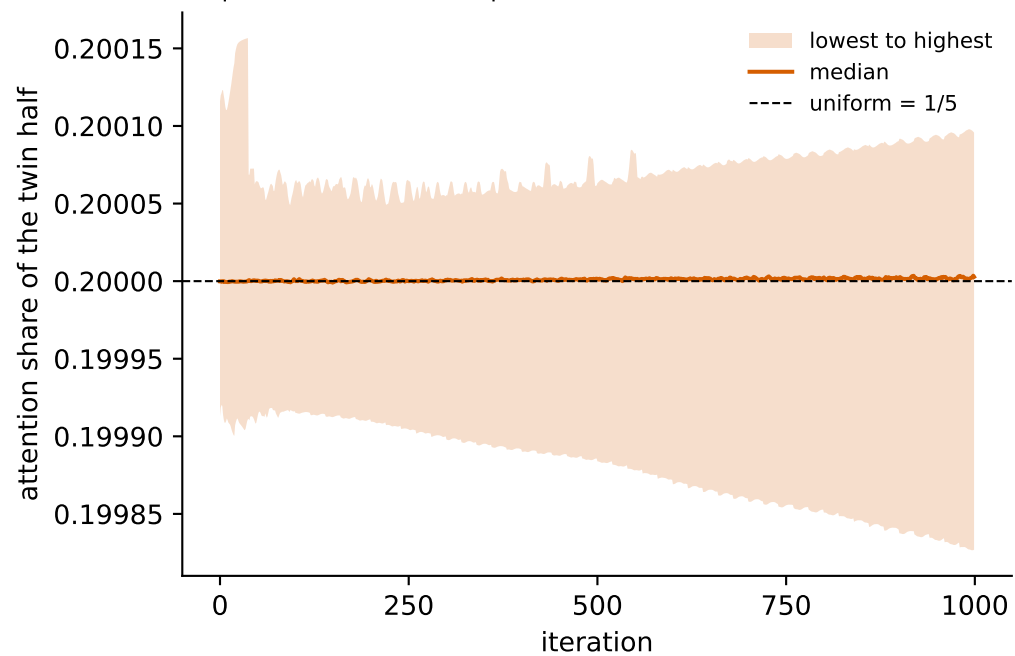
Share given to the twin half over the run, edges with 5 incoming neighbors (2888 twin rows in total, 50 seeds; a seed drops out once its run stops)
