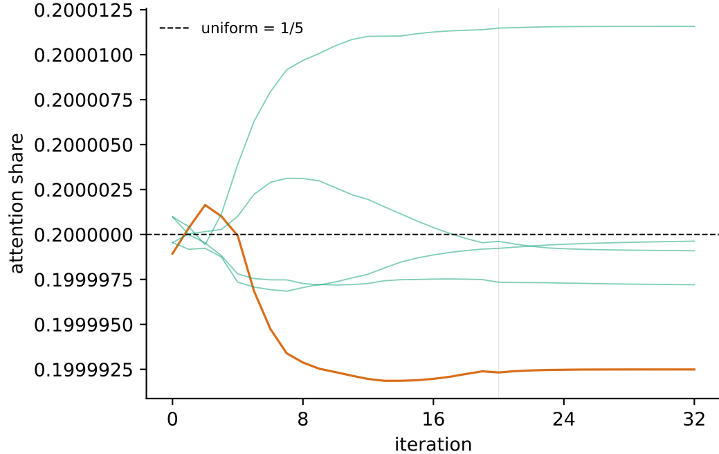
All 5 incoming shares of one edge (seed 0, x2 to f26; red = twin half)
