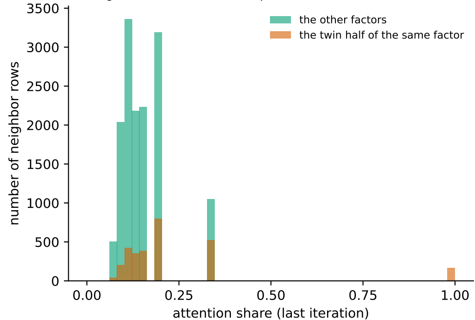
Share given to the twin half compared with the other factors
