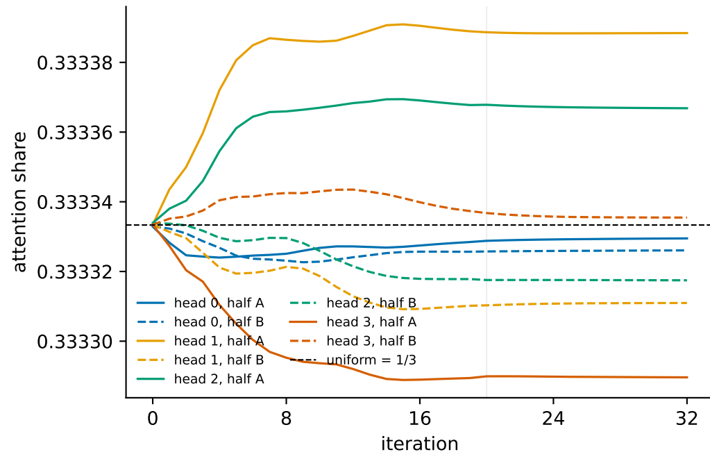
The pair whose shares drifted apart the most (seed 0, x9 to f29, halves of f79; solid = half A, dashed = half B)
