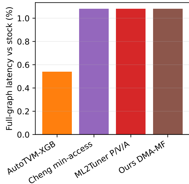
ResNet18 transfer after safe fallback
