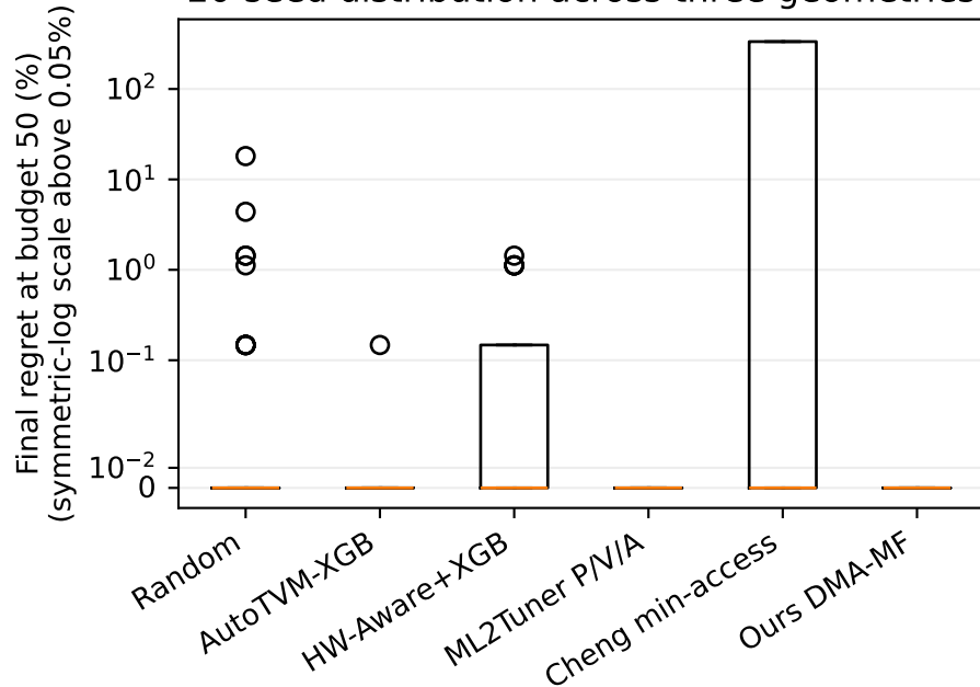
20-seed distribution across three geometries
