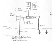
ELECTRICAL RISER DIAGRAM Typical of each tenant space (2' x 10')
