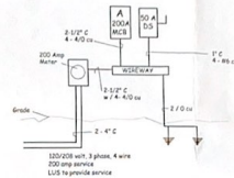
ELECTRICAL RISER DIAGRAM Typical of each tenant space (5 units)
