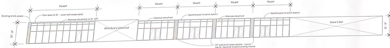
1/8" Front Elevation (Johnston Street)
