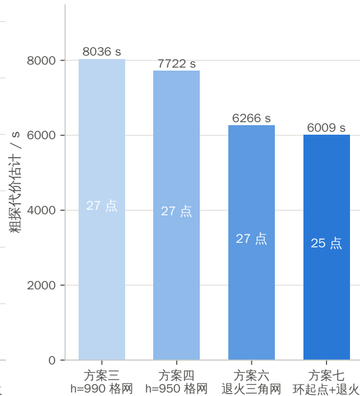
(b) 粗探代价 = 巡回/5 + 点数×20×5 s
