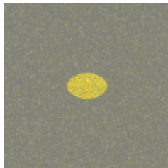
Canonical compact
