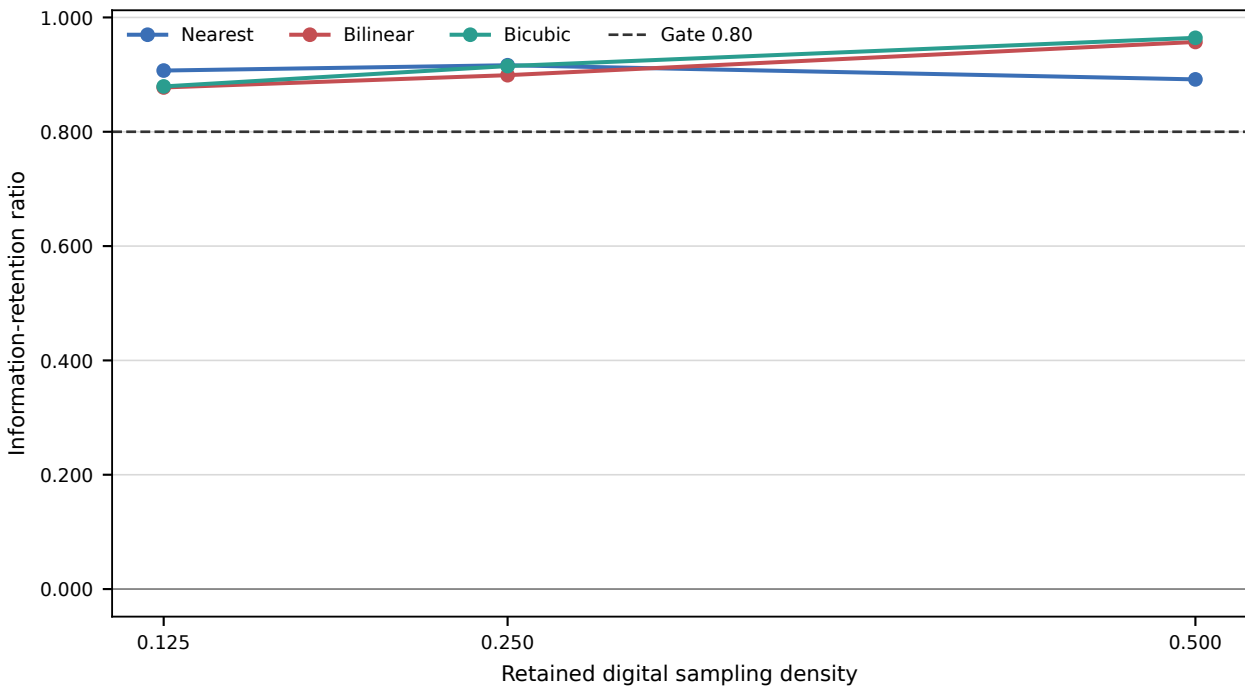
Sparse C-scan grid: retained CAI information
