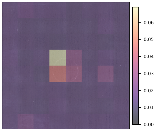
N last-layer query (self=0.013)
