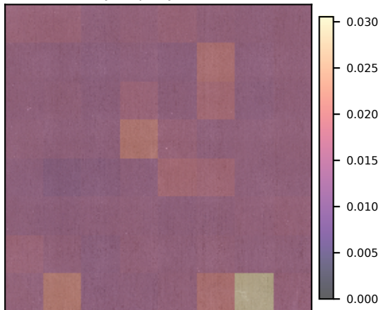
N last-layer query (self=0.029)
