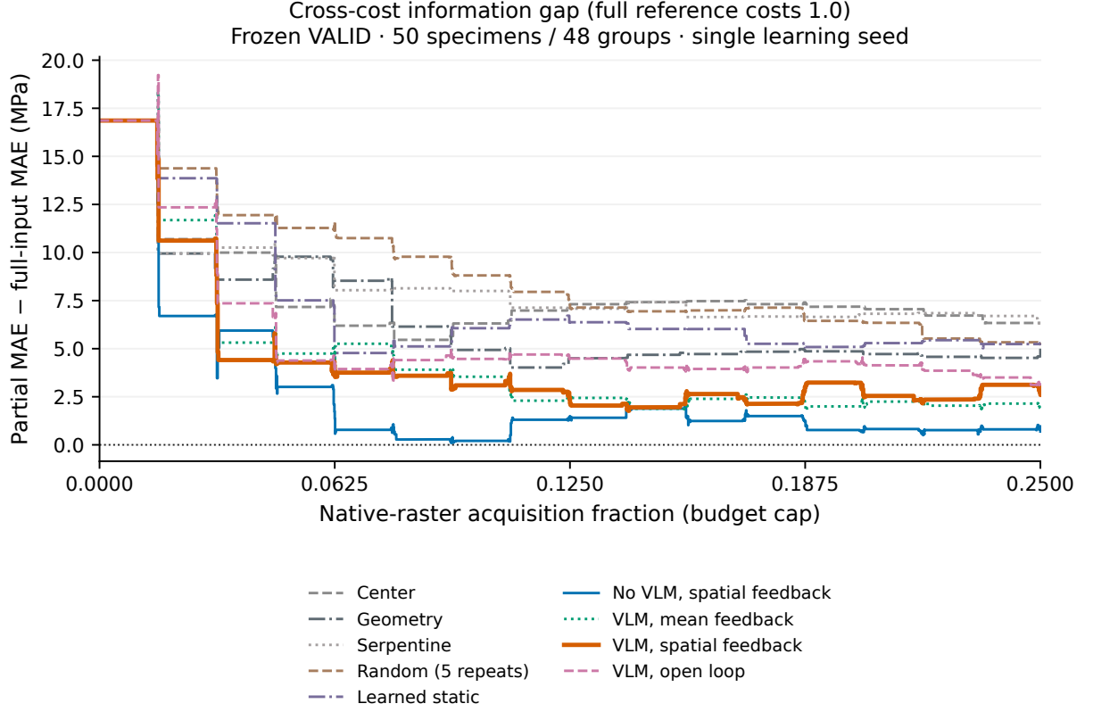
Figure S3: MAE difference from the common predictor’s complete-input reference. Zero is a quality-gap reference, not a prespecified noninferiority margin. No partial method reaches complete-input MAE in the observed range.
