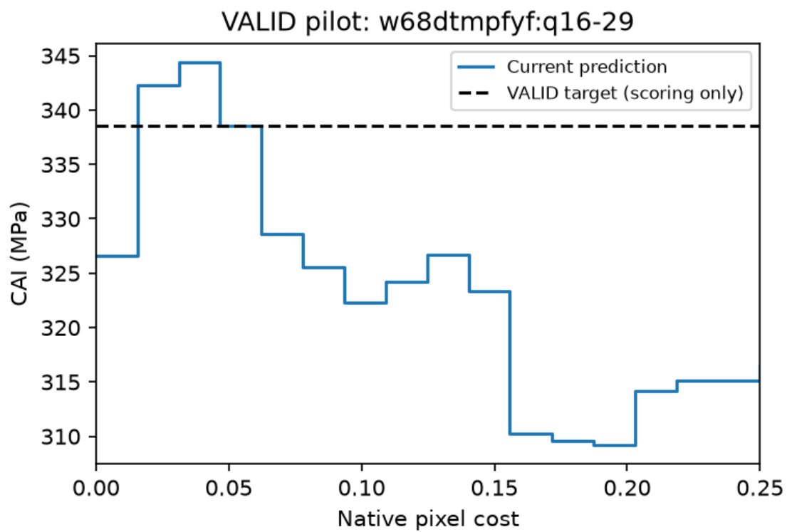
Figure S9: w68dtmpfyf: q16-29 — prediction. Frozen final acquisition state or prediction trajectory; higher-error outcomes remain visible.
