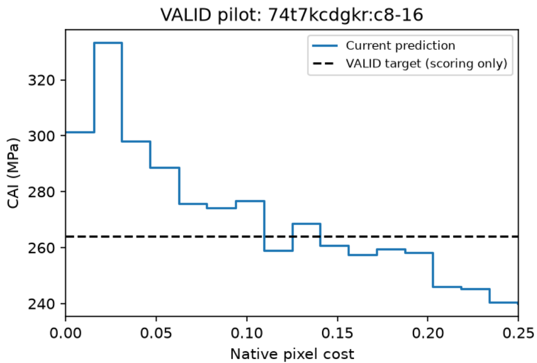
Figure S6: 74t7kcdgkr: c8-16 — prediction. Frozen final acquisition state or prediction trajectory; higher-error outcomes remain visible.
