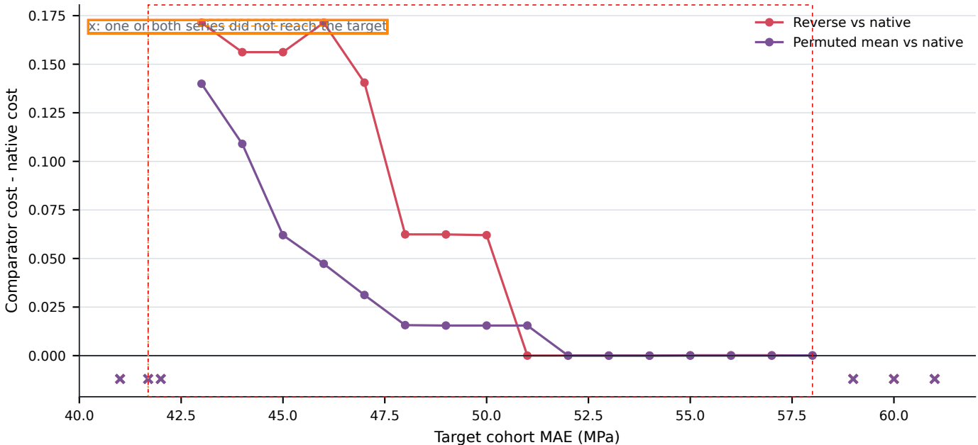
Matched-quality acquisition savings preserve crossings and unreached targets
