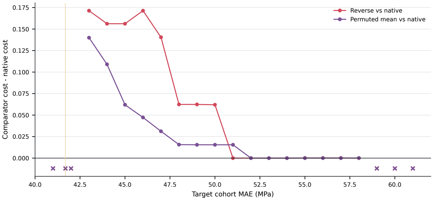
Matched-quality acquisition savings preserve crossings and unreachable targets
