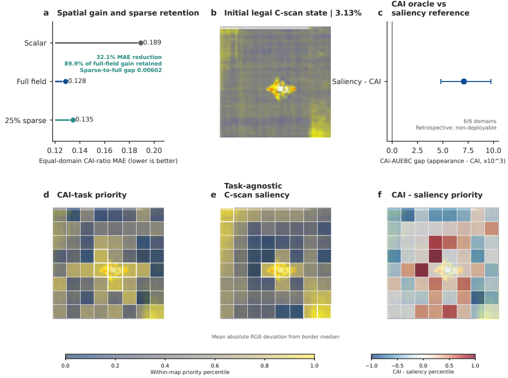
Figure 2: What ultrasonic information matters for CAI? (a) Equal-domain CAI-ratio MAE for matched scalar, full spatial field, and registered 25% sparse field. (b) Hash-verified initial legal C-scan state for specimen c8-2; teal marks measured native-raster positions. (c) CAI oracle versus the preregistered task-agnostic appearance-saliency reference under the common registered acquisition protocol. (d,e) Within-map priority percentiles for CAI-task value and task-agnostic C-scan saliency on the same initial state and legal 8 \times 8 action grid; white outlines mark the five highest-priority cells. Saliency is the mean absolute RGB deviation of newly revealed samples from the specimen-specific border median and uses no CAI outcomes. (f) Paired CAI-minus-saliency percentile difference, not raw utility or a causal material map. Both oracles are retrospective and non-deployable.
