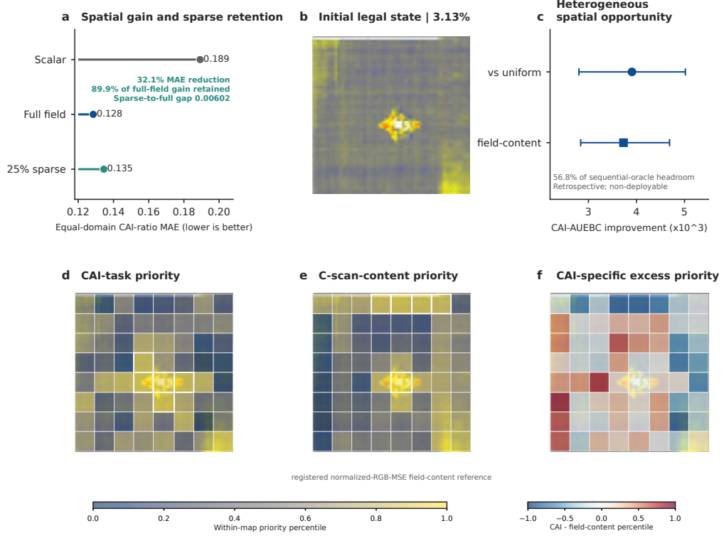
Figure 2: What ultrasonic information matters for CAI? (a) Equal-domain CAI-ratio MAE for matched scalar, full spatial field, and registered 25% sparse field. (b) Hash-verified initial legal state for specimen c8-2; teal marks measured native-raster positions. (c) Retrospective mechanical-oracle opportunity relative to uniform acquisition and the registered field-content reference. (d,e) CAI-task and C-scan-content priority percentiles on the same state and legal action grid; white outlines mark the five highest-priority cells. The field-content reference is operationalized by the registered normalized-RGB-MSE reconstruction objective. (f) Paired CAI-specific excess priority, not raw utility or a causal material map. Oracles are retrospective and non-deployable.
