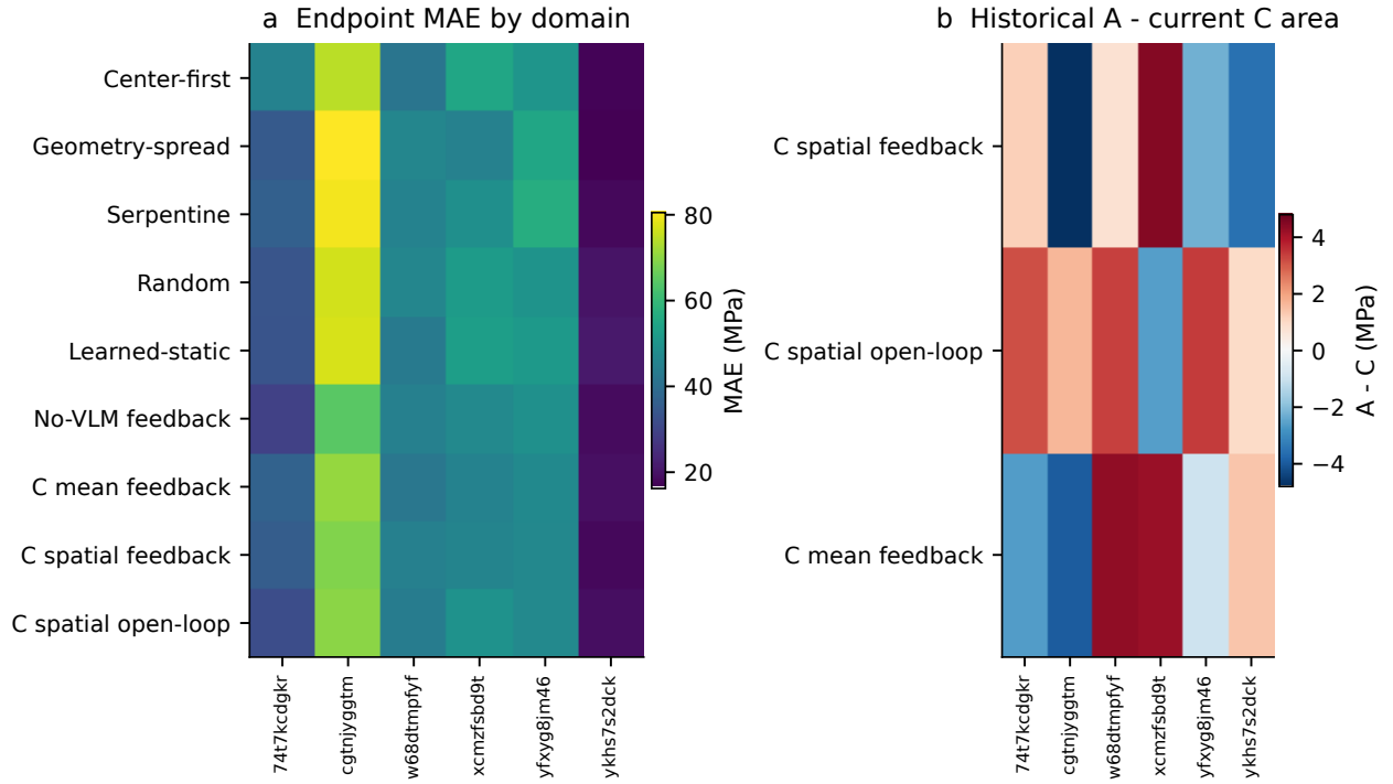
Figure 4: Endpoint performance by domain and historical-A-minus-current-C trajectory area for the three retrained policies.
