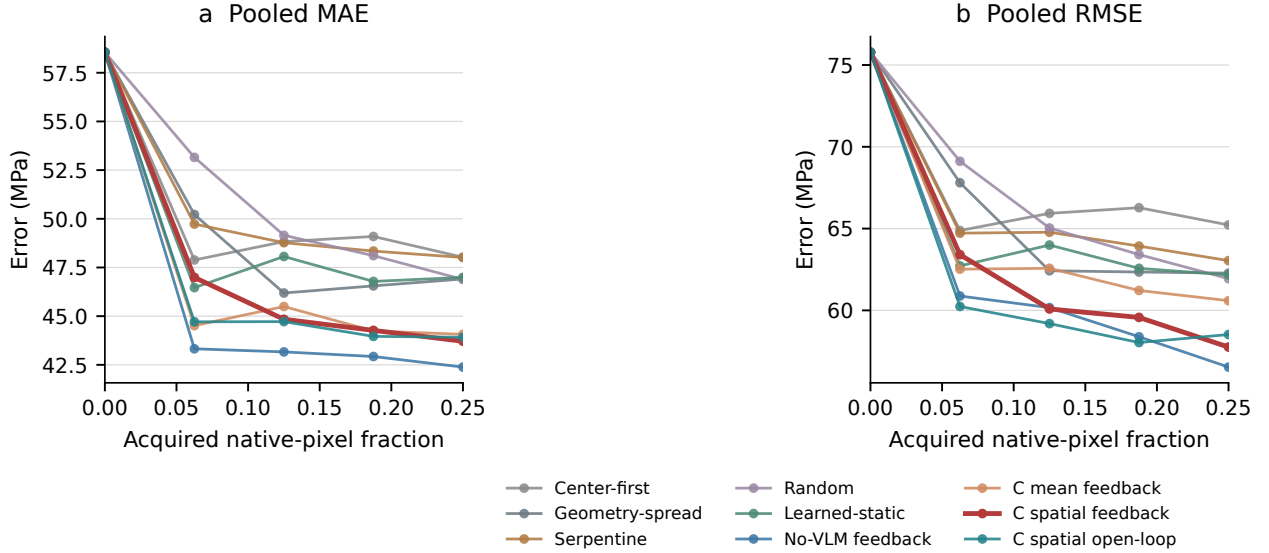
Figure 2: Current C MAE and RMSE along the five frozen acquisition caps. Curves retain observed reversals and use no smoothing.
