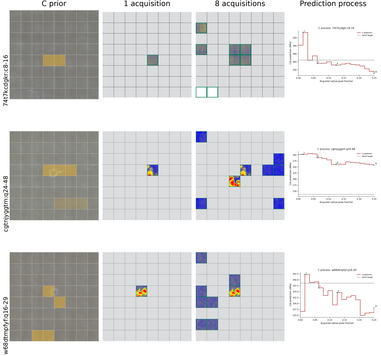
Figure 6: Current C acquisition progression for the three fixed validation cases. Panels show the C prior, acquired states and saved prediction paths.
