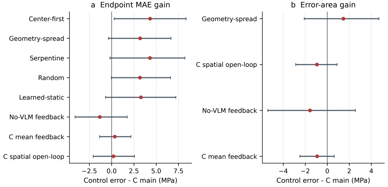
Figure 3: Paired endpoint and trajectory-area contrasts. Positive values favour current C spatial feedback; all signs and intervals are retained.
