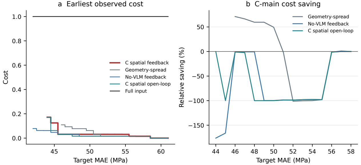
Figure 7: Earliest observed costs and current-main savings across the complete empirical MAE target grid.
