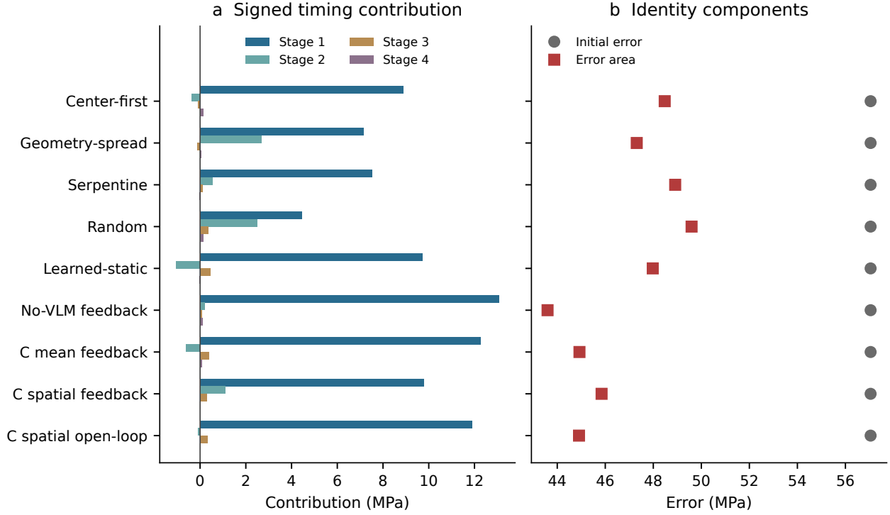
Figure 5: Signed timing-weighted contributions for all nine methods. Negative values and unequal initial-error terms are retained.
