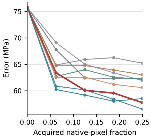
b Pooled RMSE
