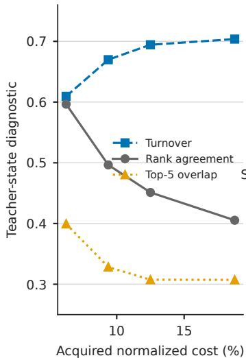
(a) Value evolves with state
