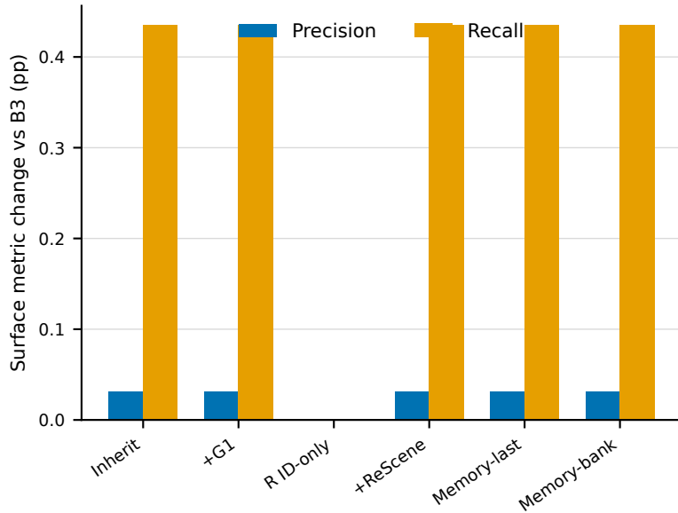
(b) Local recovery raises recall
