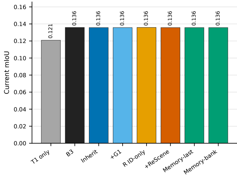
(a) B3 remains the DEV winner
