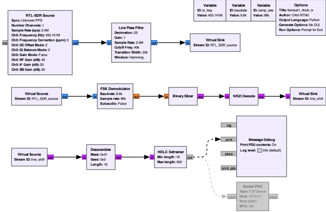
Figure 1: Recommended GNU Radio receiver pipeline for FramSat-1 using an RTL-SDR dongle (sampling at 2.4 MSps and decimated to 96 kSps).
