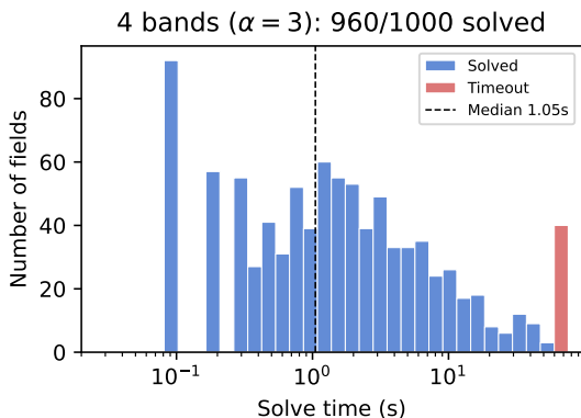
Figure 1: Solve time histogram for the 4-band configuration ( \alpha = 3 ). Timeouts at 60 s are shown in red. The dashed line marks the median solve time.
