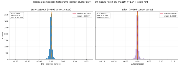
Figure 8: Histograms of the signed RA and Dec residual components for the 995 correct cases at R = 1^\circ (error \leq 1'' ). Both centred at zero to within 2 mas; \sigma_{\Delta\alpha \cos \delta} = 32 mas, \sigma_{\Delta\delta} = 46 mas. Larger Dec scatter reflects TAN-WCS fitting geometry.
