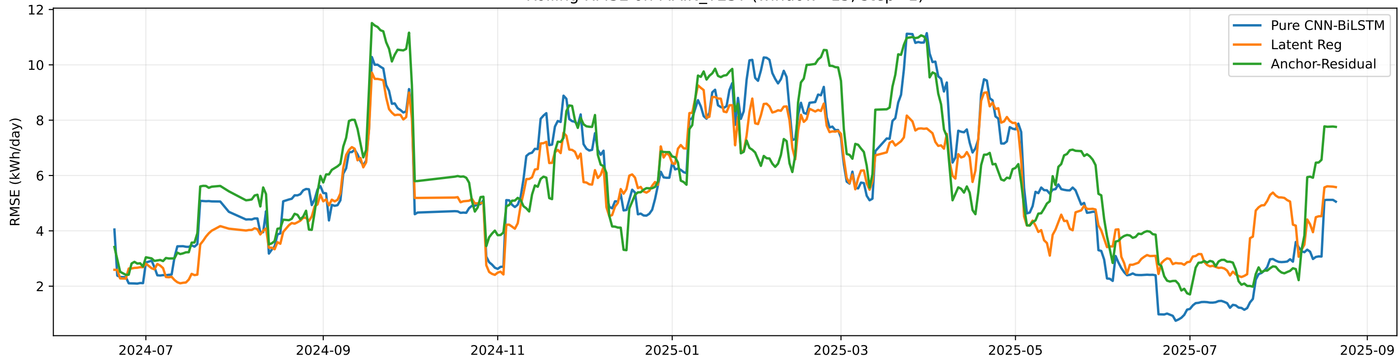
Rolling RMSE on PRED_TEST (window=15, step=1)
