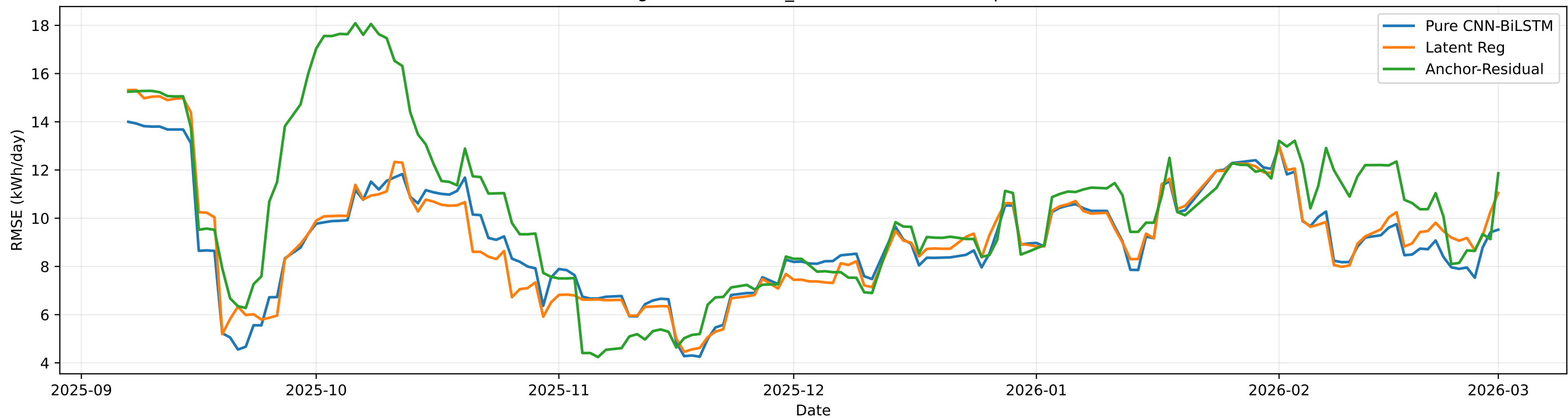
Rolling RMSE on PRED_TEST (window=15, step=1)
