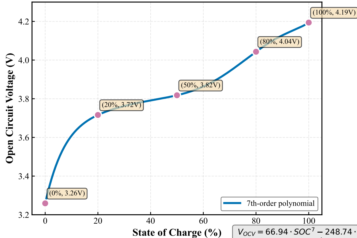
(a) OCV-SOC Characteristic
