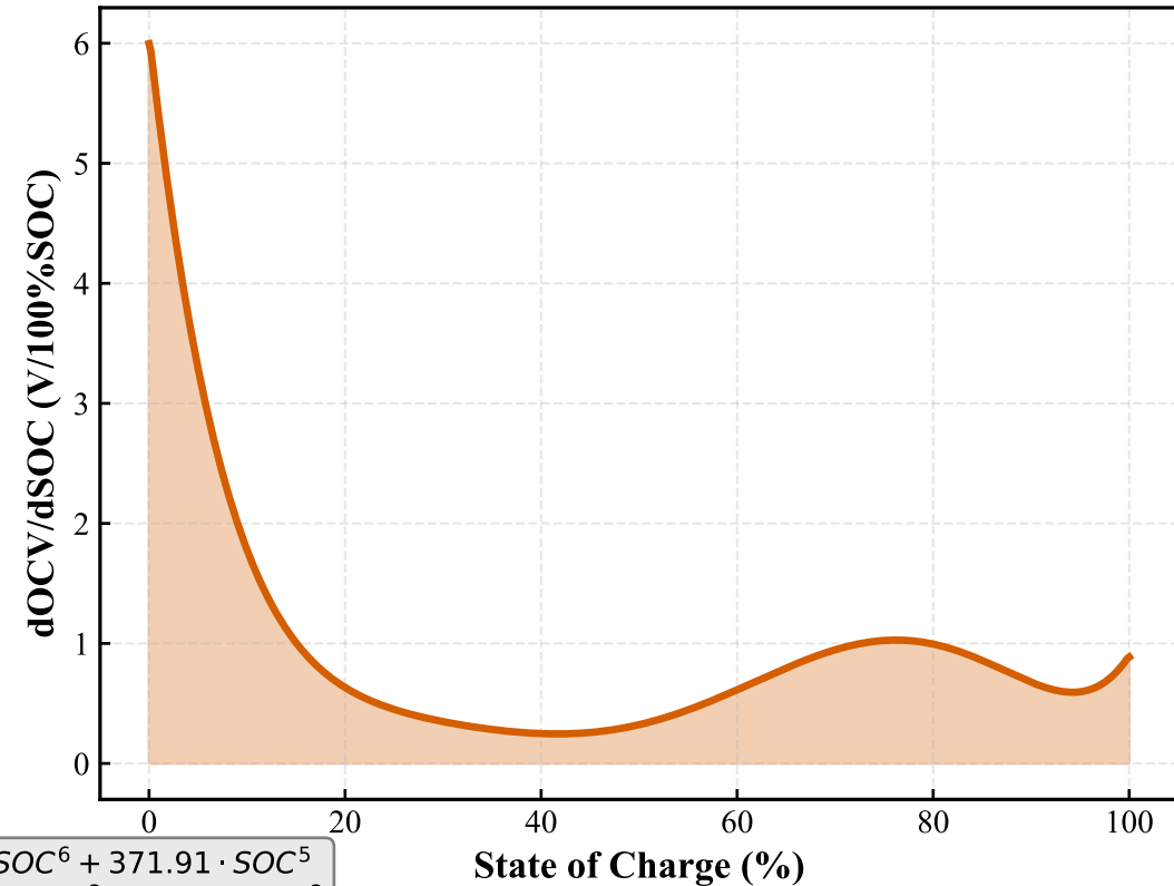
(b) OCV Sensitivity to SOC
