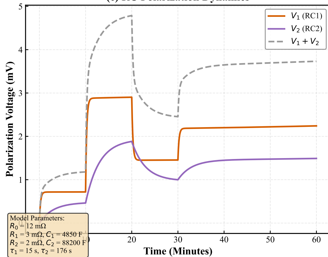
(c) RC Polarization Dynamics
