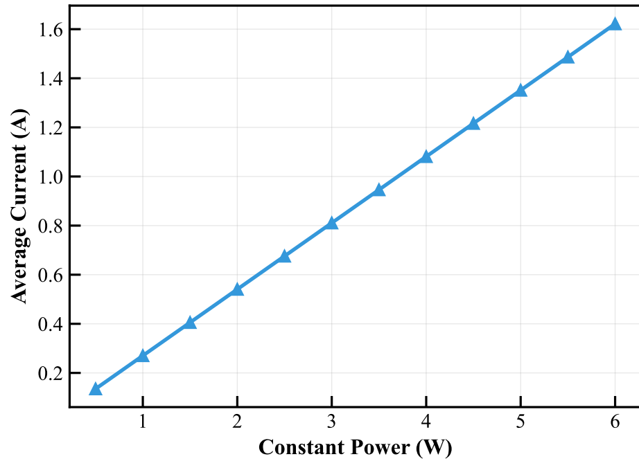
Average Current vs Power
