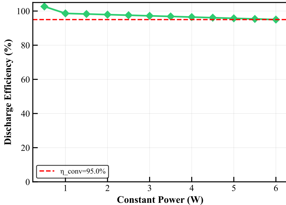
Efficiency vs Power
