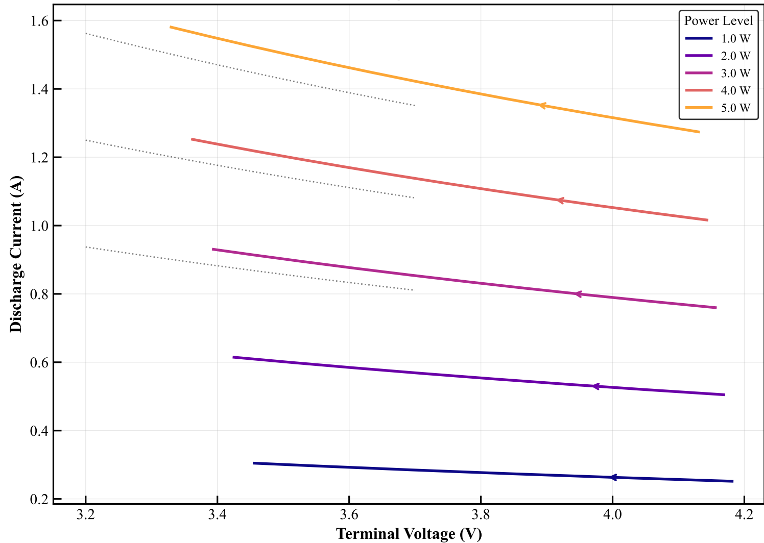
Current-Voltage Characteristics
